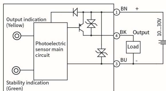
PNP
