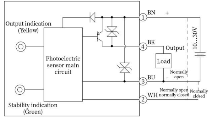
PNP
