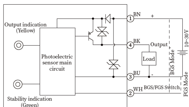
PNP
